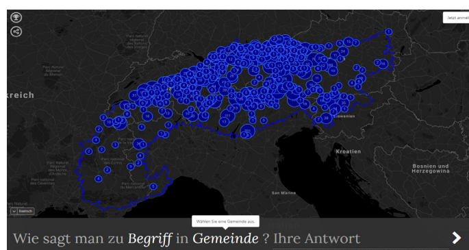
Figura 3: Crowdsourcing Tool
